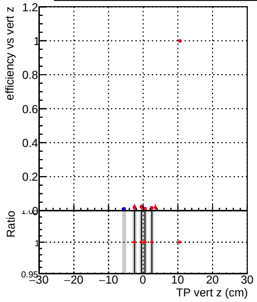
Efficiency vs TP vert z Legend: DQM_old (blue), DQM_V0001_R0000000001_Global_CMSSW_X_Y_Z_RECO (red)
