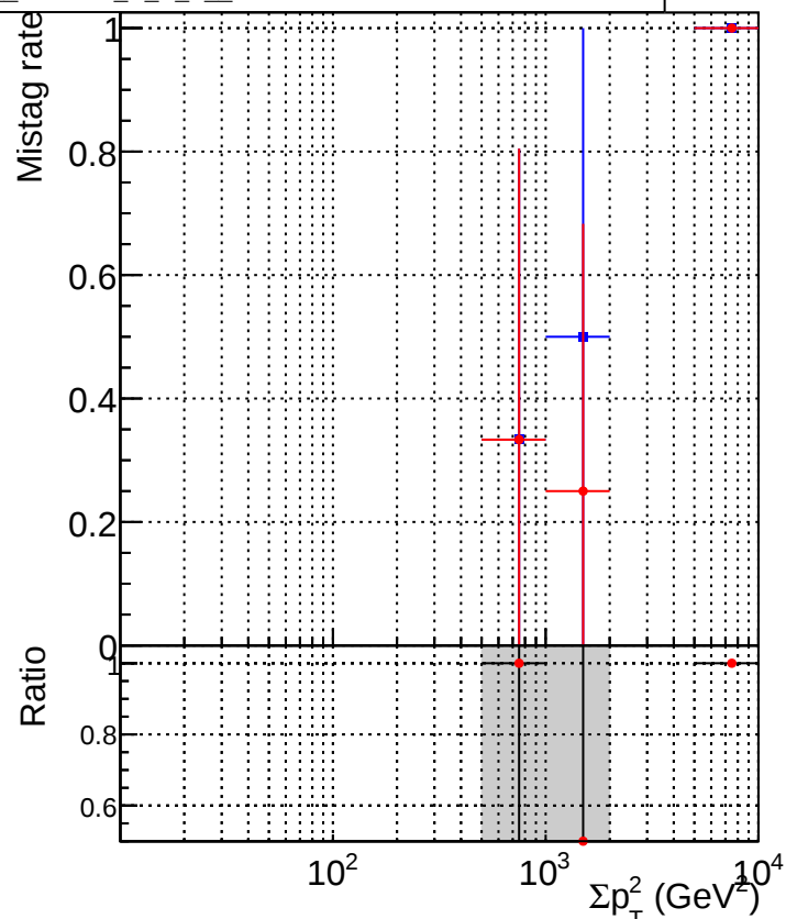
■ DQM_old ● DQM_V0001_R000000001_Global_CMSSW_X_Y_Z_RECO
