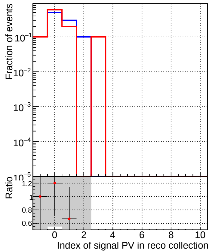
■ DQM_old ● DQM_V0001_R000000001_Global_CMSSW_X_Y_Z_RECO
