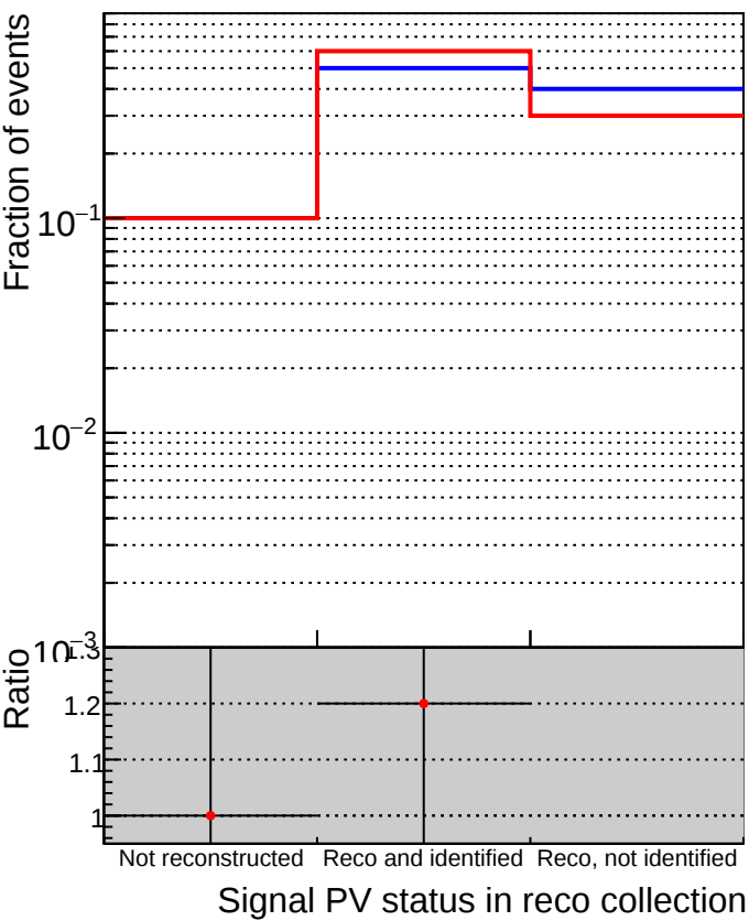
■ DQM_old ● DQM_V0001_R000000001_Global_CMSSW_X_Y_Z_RECO
