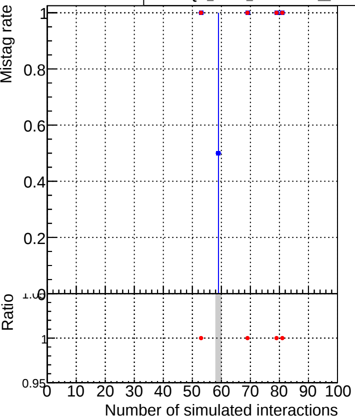
■ DQM_old ● DQM_V0001_R000000001_Global_CMSSW_X_Y_Z_RECO
