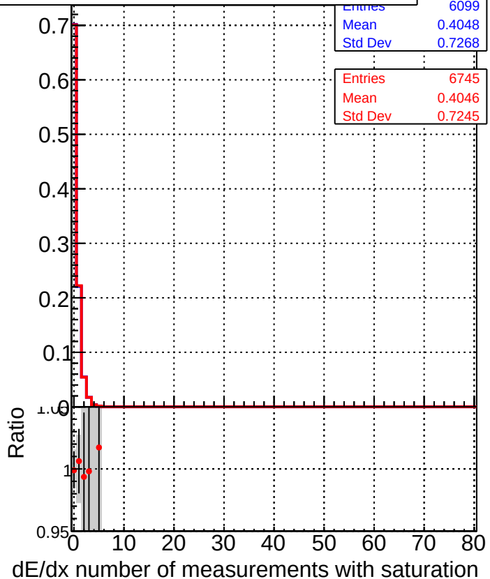
Legend: DQM_old (blue line with squares), DQM_V0001_R000000001_Global_CMSSW_X_Y_Z_RECO (red line with circles)
