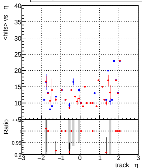
mean hits vs \eta Legend: DQM_old (blue line), DQM_V0001_R000000001_Global_CMSSW_X_Y_Z_RECO (red line)
