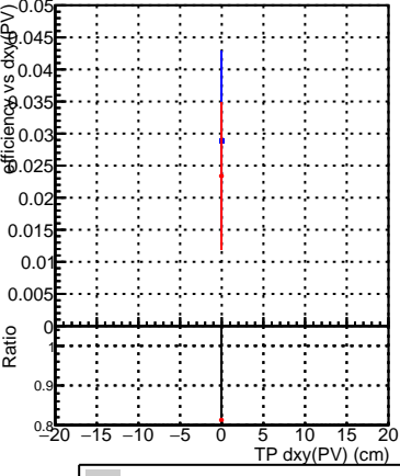
Efficiency vs Dxy(PV) DQM_old DQM_V0001_R00000001_Global_CMSSW_X_Y_Z_RECO
