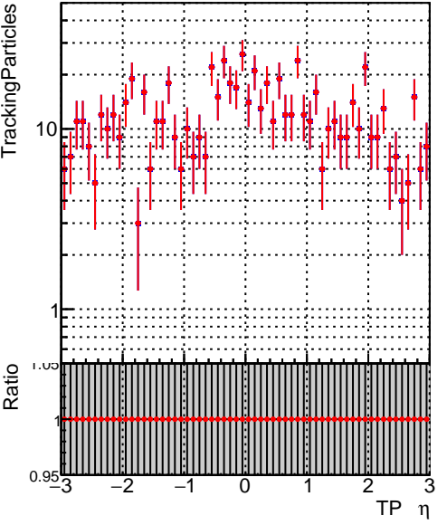
— DQM_old — DQM_V0001_R000000001_Global_CMSSW_X_Y_Z_RECO
