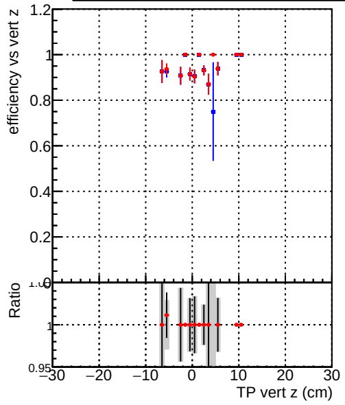
Efficiency vs vert z Legend: DQM_old (blue line), DQM_V0001_R000000001_Global_CMSSW_X_Y_Z_RECO (red line)
