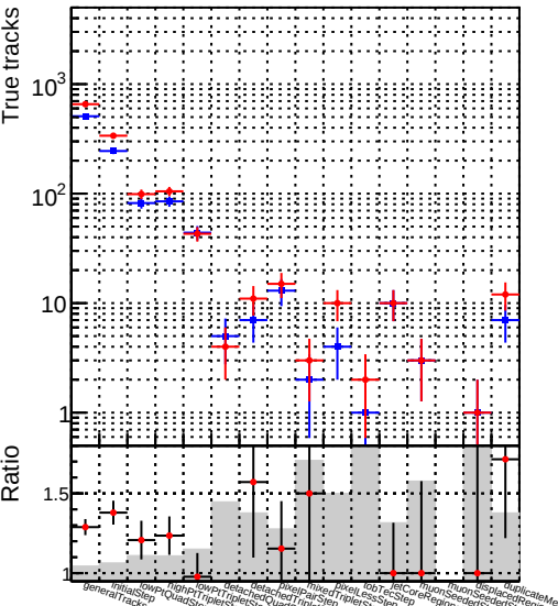
Number Legend: DQM_old DQM_V0001_R0000000001_Global_CMSSW_X_Y_Z_RECO
