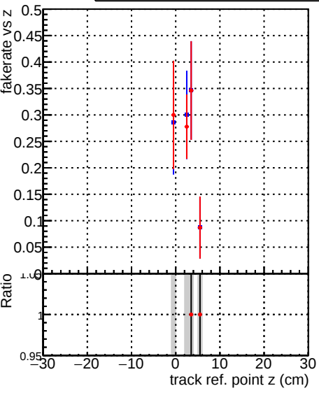
Fake rate vs track ref. point z (cm) Legend: DQM_old (blue squares), DQM_V0001_R000000001_Global_CMSSW_X_Y_Z_RECO (red circles)
