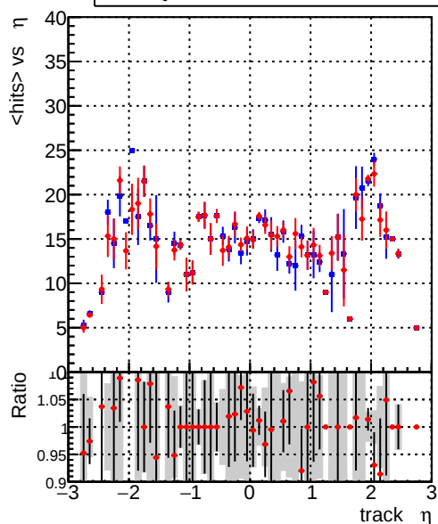
mean hits — DQM_old — DQM_V0001_R000000001_Global_CMSSW_X_Y_Z_RECO
