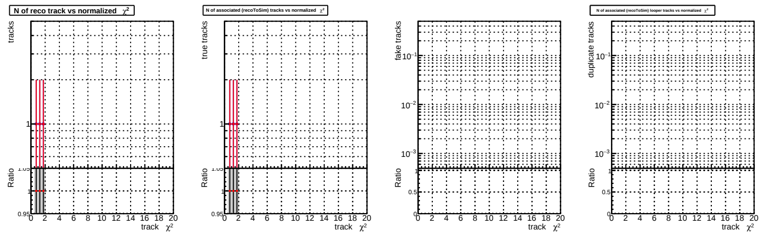
N of reco track vs. \chi^2 DQM old DQM V0001_R000000001_Global_CMSSW_X_Y_Z_RECO
