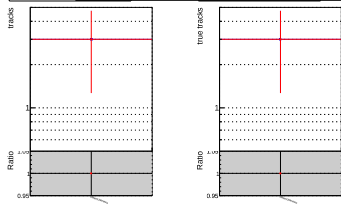
N of reco track vs. \chi^2 DQM old DQM V0001_R000000001_Global_CMSSW_X_Y_Z_RECO
