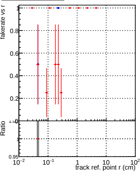
—■ DQM_old —● DQM_V0001_R000000001_Global_CMSSW_X_Y_Z_RECO
