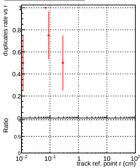
—■ DQM_old —● DQM_V0001_R000000001_Global_CMSSW_X_Y_Z_RECO
