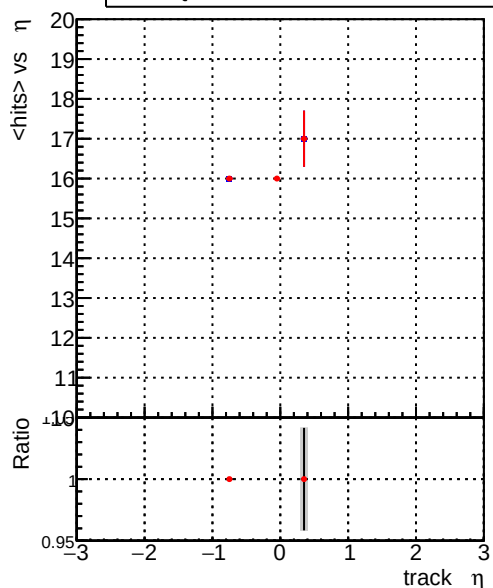
mean hit — DQM_old — DQM_V0001_R0000000001_Global_CMSSW_X_Y_Z_RECO
