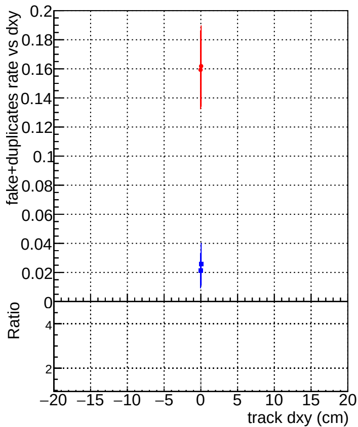
DQM_old DQM_V0001_R000000001_Global_CMSSW_X_Y_Z_RECO
