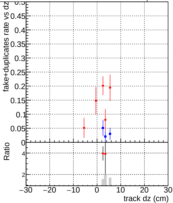
DQM_old DQM_V0001_R000000001_Global_CMSSW_X_Y_Z_RECO
