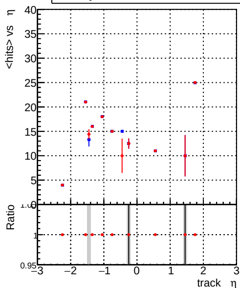
mean hit Legend: DQM_old (blue line), DQM_V0001_R000000001_Global_CMSSW_X_Y_Z_RECO (red line)
