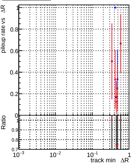
Fake rate vs \Delta R (track, jet) Duplicates Rate vs \Delta R (track, jet) Pileup rate vs \Delta R (track, jet) Legend: DQM_old (blue line with error bars), DQM_V0001_R000000001_Global_CMSSW_X_Y_Z_RECO (red line with error bars)
