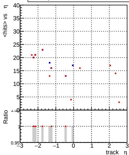
mean hit \eta Legend: DQM_old (blue line), DQM_V0001_R000000001_Global_CMSSW_X_Y_Z_RECO (red line)
