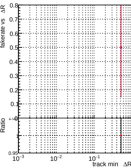
DQM_old DQM_V0001_R000000001_Global_CMSSW_X_Y_Z_RECO
