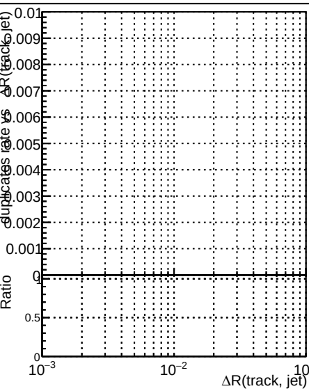
—●— DQM_old —●— DQM_V0001_R000000001_Global_CMSSW_X_Y_Z_RECO
