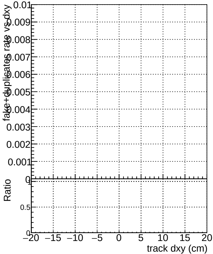
DQM_old DQM_V0001_R000000001_Global_CMSSW_X_Y_Z_RECO
