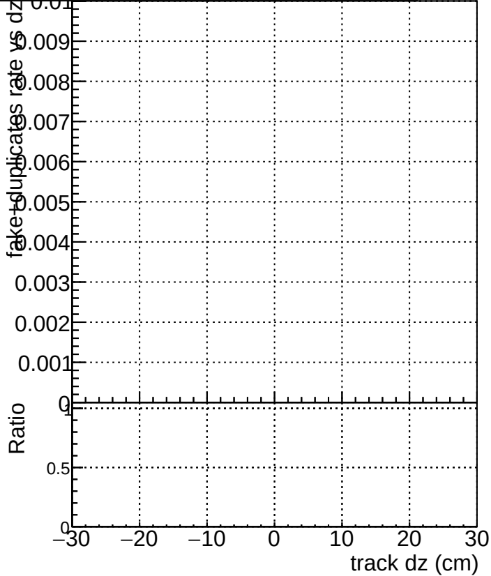
DQM_old DQM_V0001_R000000001_Global_CMSSW_X_Y_Z_RECO
