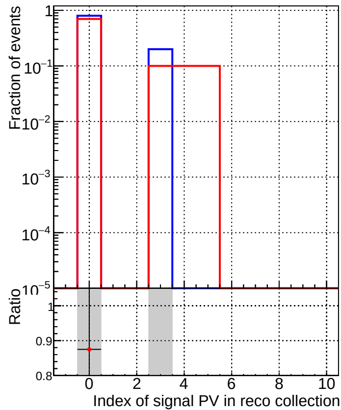
TruePVLocationIndexInRecoVertexCollection
