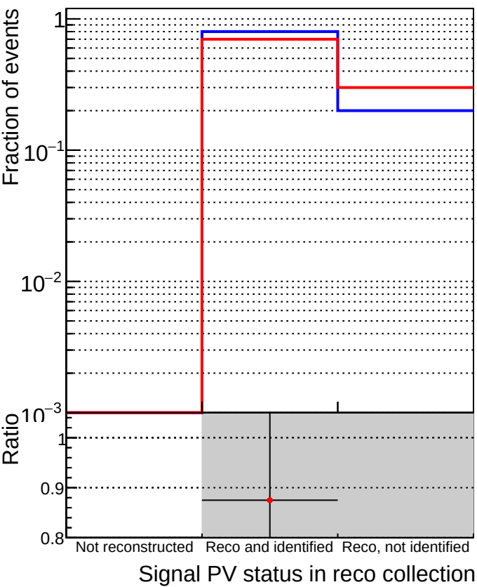
TruePVLocationIndexInRecoVertexCollectionCumulative
