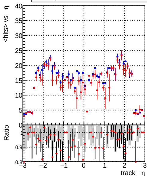
mean hits Legend: DQM_old (blue line), DQM_V0001_R000000001_Global_CMSSW_X_Y_Z_RECO (red line)
