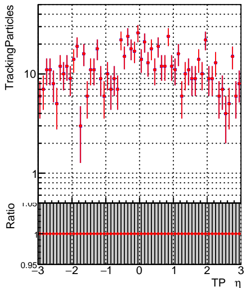
— DQM_old — DQM_V0001_R000000001_Global_CMSSW_X_Y_Z_RECO
