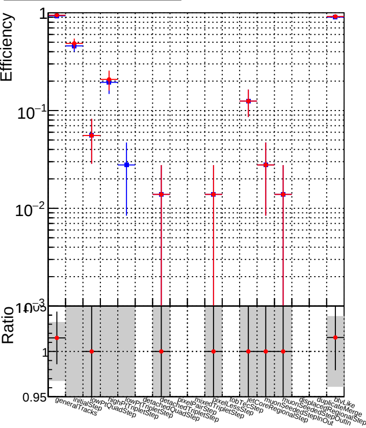
DQM_old DQM_V0001_R000000001_Global_CMSSW_X_Y_Z_RECO
