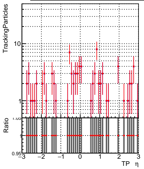
N of simulated tracks vs \eta Legend: DQM_old (blue line with error bars), DQM_V0001_R000000001_Global_CMSSW_X_Y_Z_RECO (red line with error bars)
