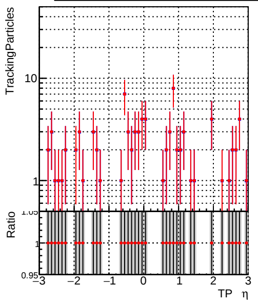
N of simulated tracks vs \eta (Legend: DQM_old, DQM_V0001_R000000001_Global_CMSSW_X_Y_Z_RECO)
