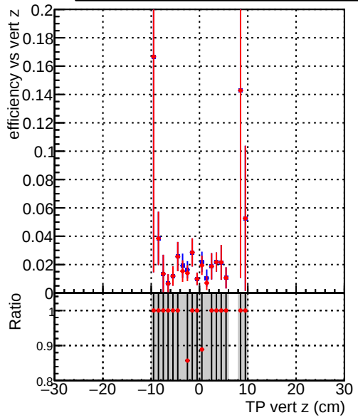
Efficiency vs TP vert z — DQM_old — DQM_V0001_R0000000001_Global_CMSSW_X_Y_Z_RECO
