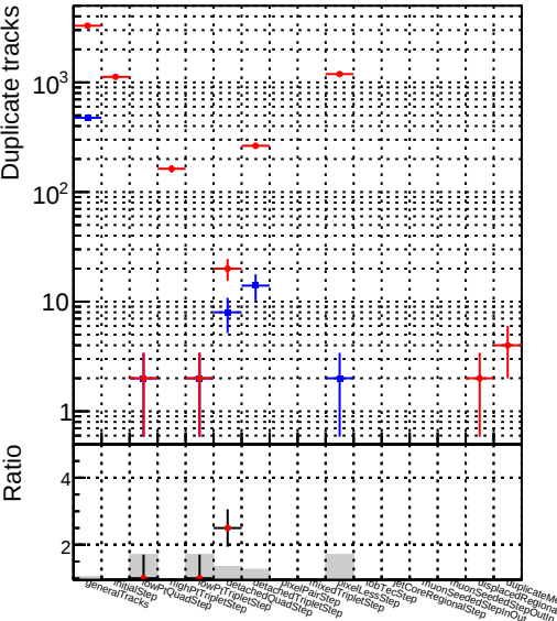
Legend: DQM_old DQM_V0001_R000000001_Global_CMSSW_X_Y_Z_RECO
