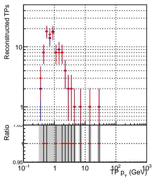
— DQM_old — DQM_V0001_R000000001_Global_CMSSW_X_Y_Z_RECO
