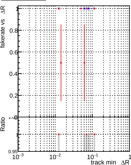
—●— DQM_old —●— DQM_V0001_R000000001_Global_CMSSW_X_Y_Z_RECO
