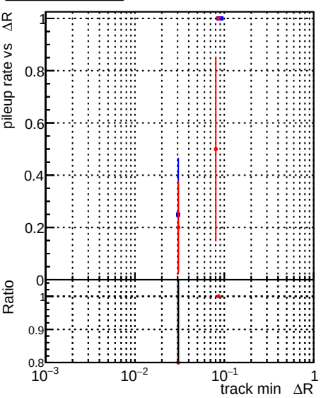
Legend: DQM_old (blue line), DQM_V0001_R000000001_Global_CMSSW_X_Y_Z_RECO (red line)
