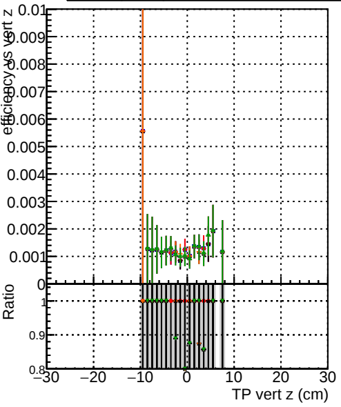
Efficiency vs vertpos Legend: original fitted cpeok sortrzz testoutlier5
