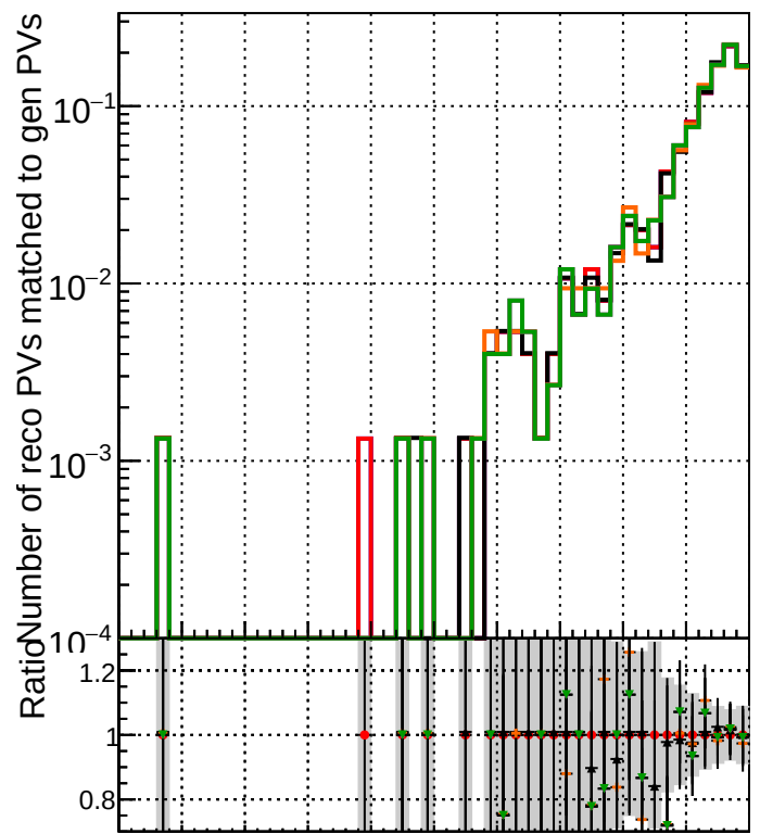
RecoPVAssoc2GenPVMatched_Purity
