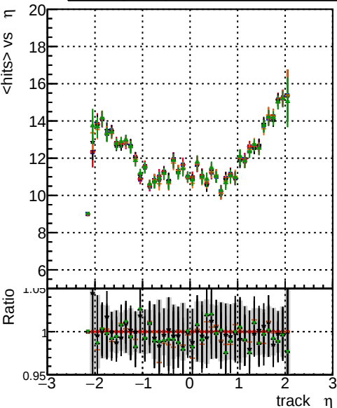
mean hits vs \eta Legend: - BQM original original vector 1000evt - BQM fitted 4 1000evt - BQM fitted 22 1000evt - BQM fit cpeok SORTZZ 1000evt - BQM fit cpeok SORTZZ TESTOUTLIER5 1000evt
