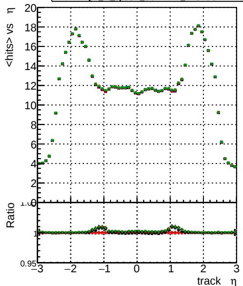
mean hits vs \eta Legend: - BOW original vector 1000evt - BOW fitted 1000evt - BOW fit cpeok SORTRZZ 1000evt - BOW fit cpeok SORTRZZ TESTOUTLIER5 1000evt
