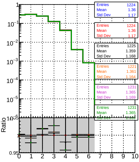
mean hits vs \eta Legend: - BOW original original vector 1000evt - BOW fitted 4 1000evt - BOW fitted 2 1000evt - BOW fitted 1 1000evt - BOW fitted 0 1000evt - BOW fitted 0 SORTRZZ 1000evt - BOW fitted 0 TESTOUTLIER5 1000evt
