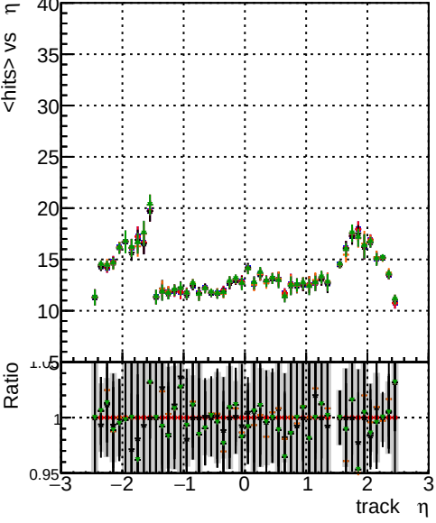
mean hits vs \eta Legend: - BOW original original vector 1000evt - BOW fitted 4 1000evt - BOW fitted 2 1000evt - BOW fitted 1 1000evt - BOW fitted 0 1000evt - BOW fitted 0 SORTRZZ 1000evt - BOW fitted 0 TESTOUTLIER5 1000evt
