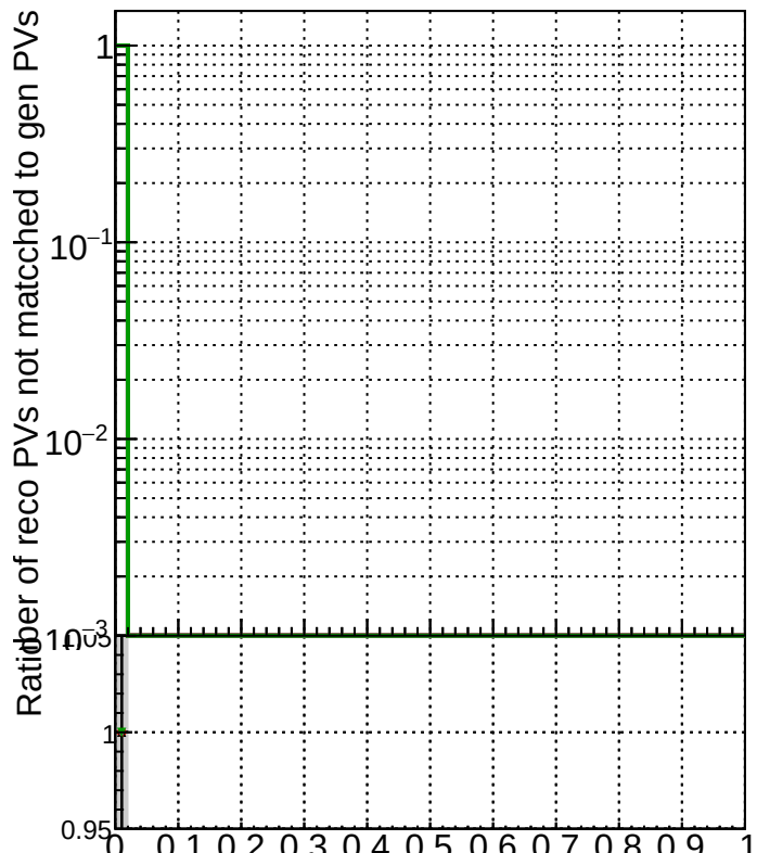
RecoPVAssoc2GenPVNotMatched_Purity
