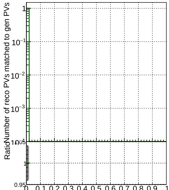
RecoPVAssoc2GenPVMatched_Purity
