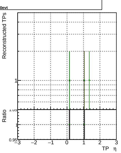
N of associated tracks (simToReco) vs eta
