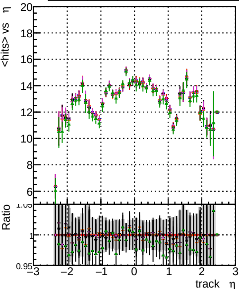
mean hits vs \eta Legend: - BOW original vector 1000evt - BOW fitted 1000evt - BOW fit cpeok SORTRZZ 1000evt - BOW fit cpeok SORTRZZ TESTOUTLIER4 1000evt
