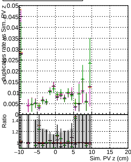
Duplicate Rate vs sim PV z
