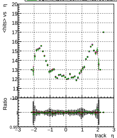
mean hits vs \eta Legend: - BOW original original vector 1000evt - BOW fitted 1000evt - BOW fit cpeok 1000evt - BOW fit cpeok SORTRZZ 1000evt - BOW fit cpeok SORTRZZ TESTOUTLIER4 1000evt
