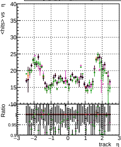
mean hits vs \eta Legend: BQM original vector 1000evt, BQM fitted 4 1000evt, BQM fitted 2 1000evt, BQM fitted 2 1000evt, BQM fitted 2 1000evt, BQM fitted 2 1000evt
