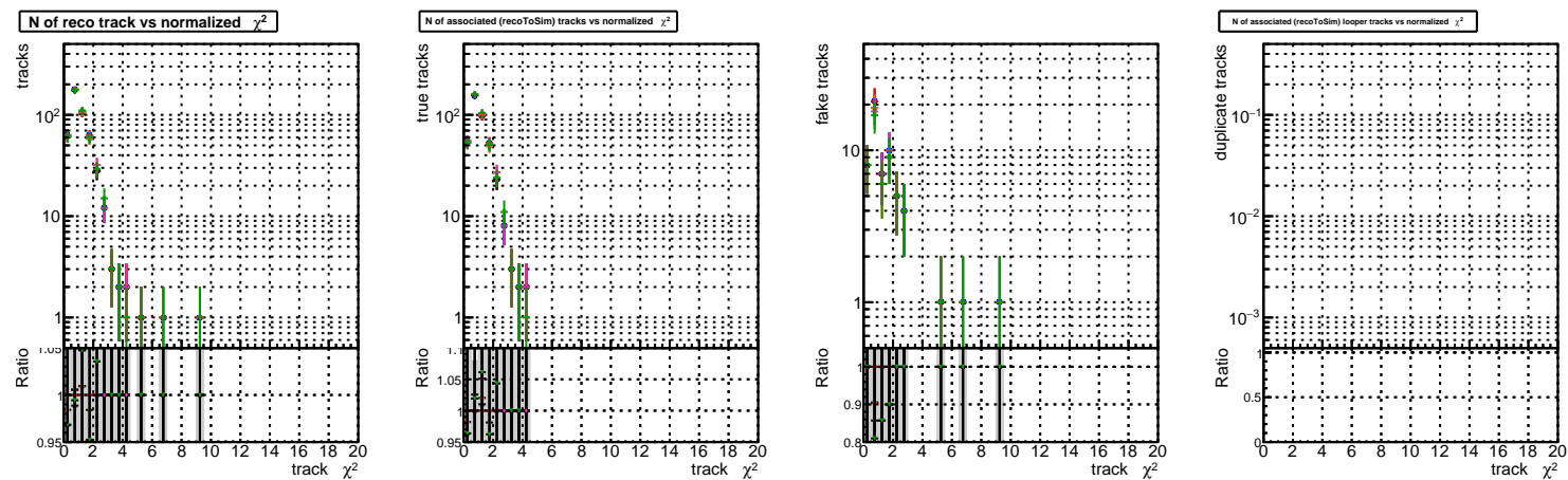
N of reco track vs. \chi^2 original original vector original 1000evt original original vector original 1000evt original original vector original 1000evt
