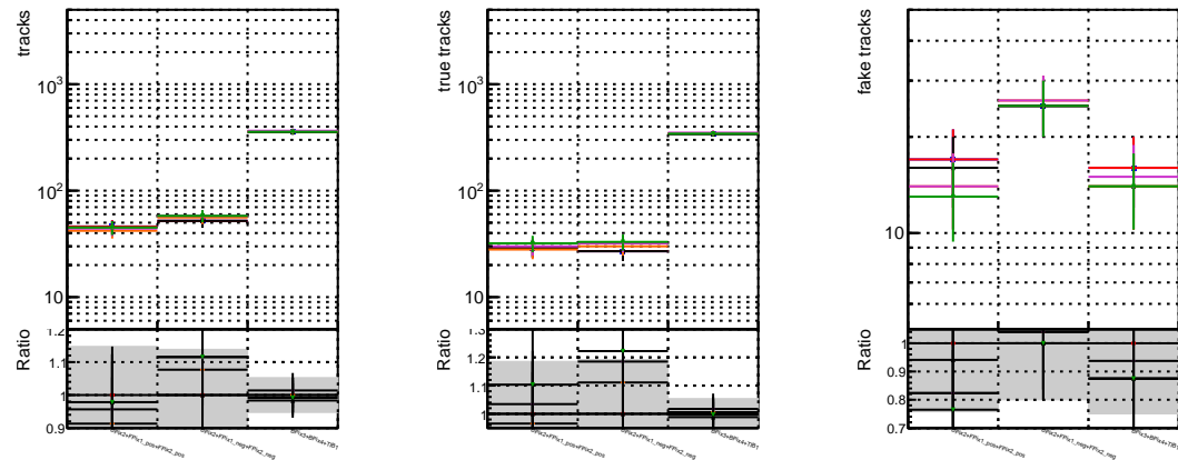
N of reco track vs. \chi^2 original original vector original 1000evt original original vector original 1000evt original original vector original 1000evt
