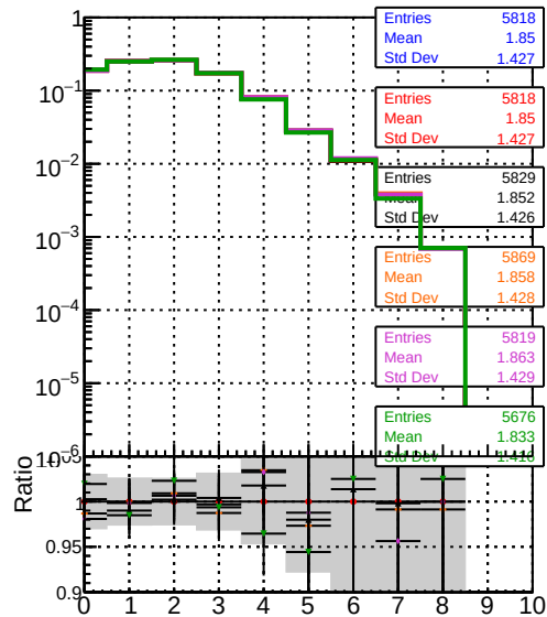
Legend: - BOM original original vector 1000evt - BOM fitted4 1000evt - BOM fit cpeok SORTZZ 1000evt - BOM fit cpeok SORTZZ TESTOUTLIER4 1000evt mean hits
