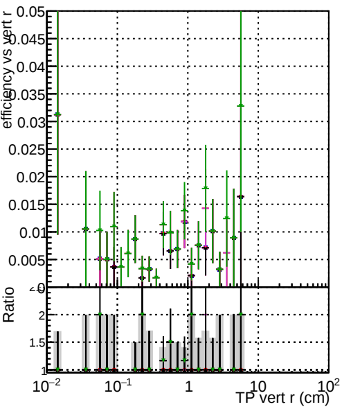
Efficiency vs TP vert r (cm) plot. Legend: original (black), original vector (blue), fitted4 (red), cpeok (green), SORTRZZ (magenta), TESTOUTLIER4 (cyan). All scenarios are for 1000evt.
