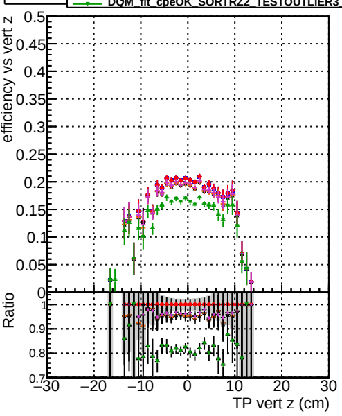
Efficiency vs. sim PV z
