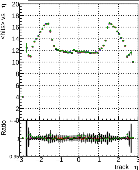
mean hits vs \eta Legend: BQM original original vector 1000evt, BQM fitted 1000evt, BQM fit cpeok SORTRZZ 1000evt, BQM fit cpeok SORTRZZ TESTOUTLIER3 1000evt
