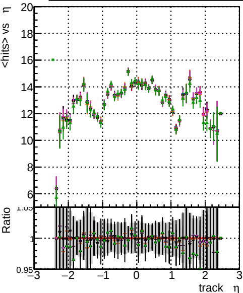
mean hits vs \eta Legend: - BOW original vector 1000evt - BOW fitted 1000evt - BOW fit cpeok SORTRZZ 1000evt - BOW fit cpeok SORTRZZ TESTOUTLIER3 1000evt
