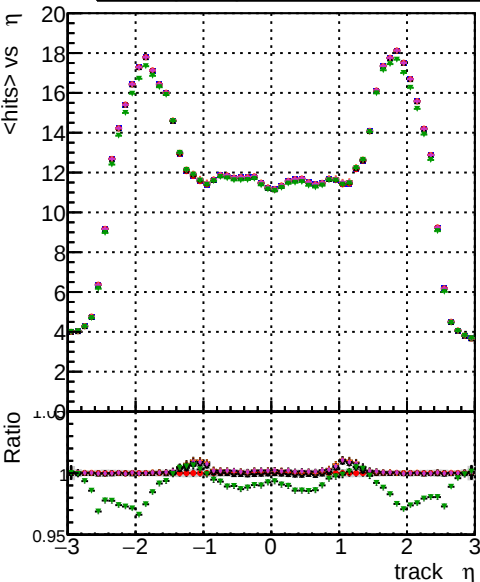
mean hits vs \eta Legend: BQM original, BQM fitted, BQM fit cpeok, BQM fit cpeok SORTRZZ, TESTOUTLIER3
