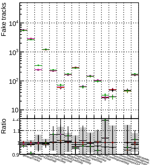
Number Color Model Method Dataset Size 1 Orange DOM fit cpeok 1000evt 2 Orange DOM fit cpeok SORTRZZ 3 Purple DOM fit cpeok SORTRZZ 4 Purple DOM fit cpeok TESTOUTLIER3 5 Green DOM fit cpeok TESTOUTLIER3
